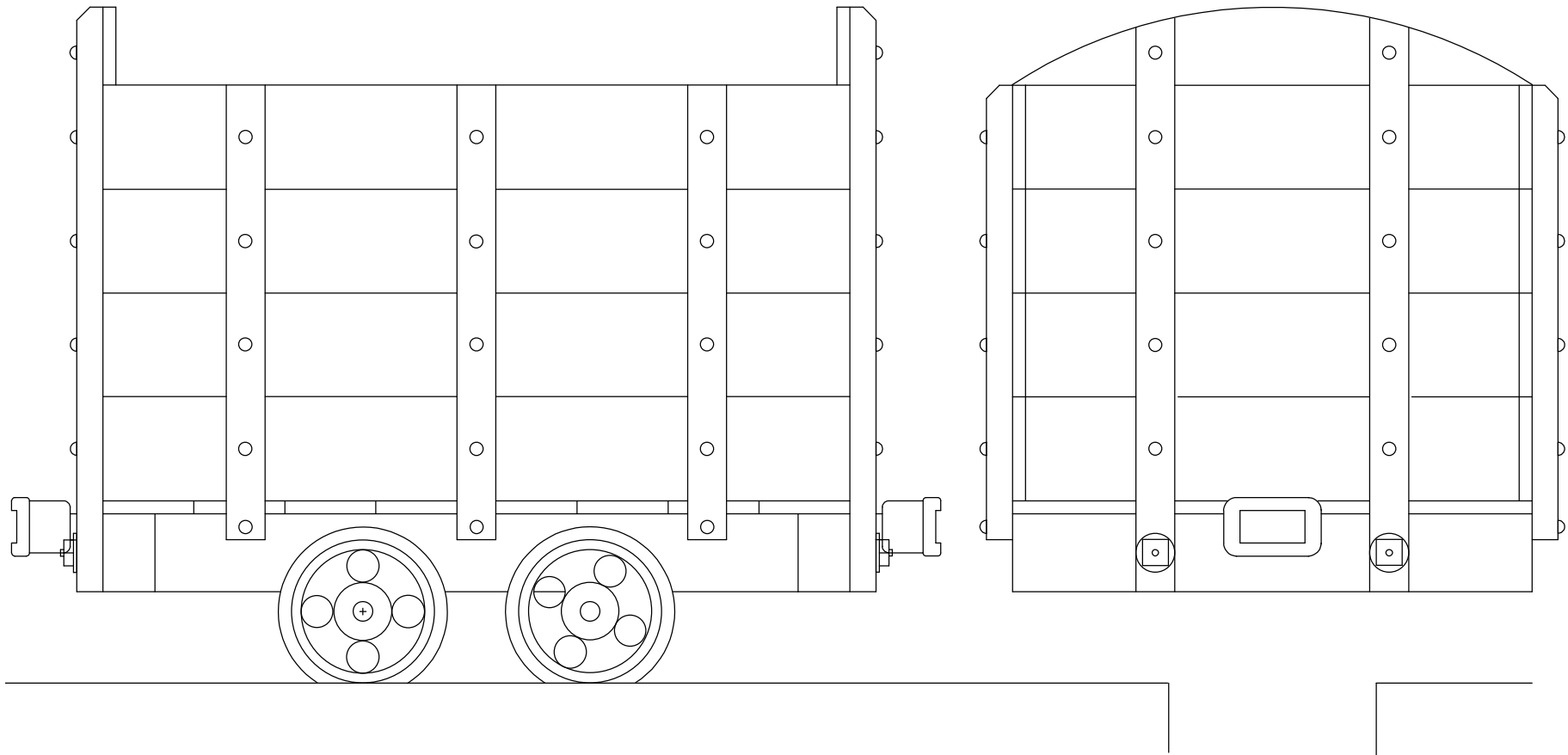
BMT Coal Wagon, Designed by Henrik Laurell Drawn by Ken Cooper March 2007
